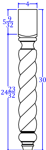
Part #6054 4" x 30"
